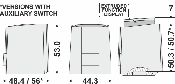
Fig. 1. Dimensions (in mm)
