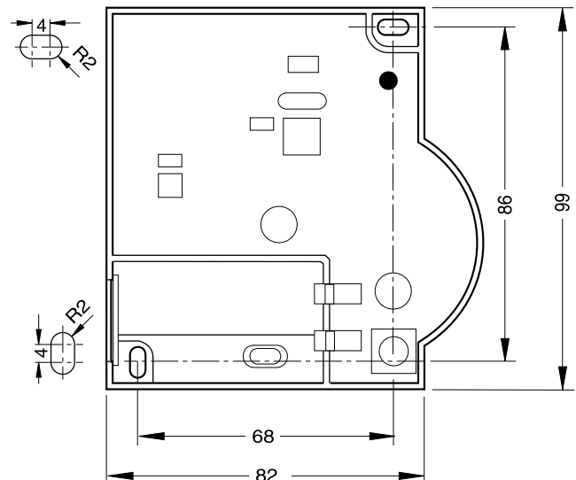
Fig. 3: Drilling scheme (measurements in mm)
